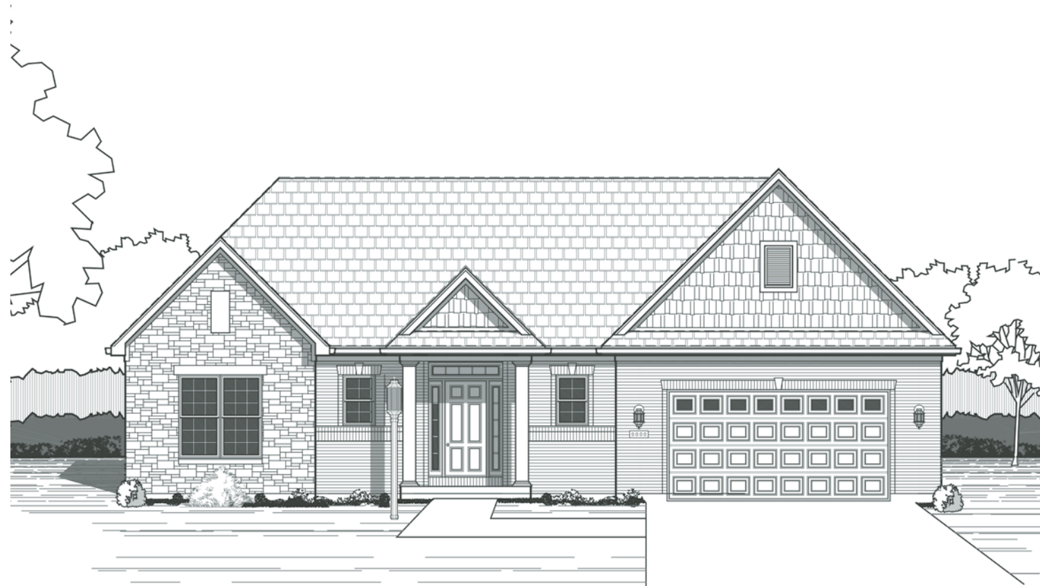
Elevation 2, Front Garage
